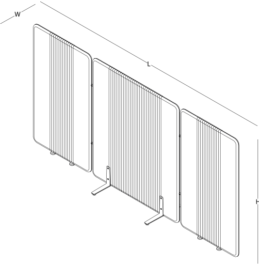
flex panel felt / acoustic felt L 285
