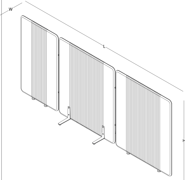
flex panel felt / acoustic felt L 325
