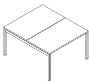
BOY42 1200 / 1410 / 740 57.2 kg
