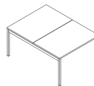
BOY32 1200 / 1610 / 740 68.3 kg
