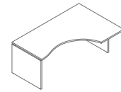
BVG18 1800 / 1200 / 740 65.5 kg
